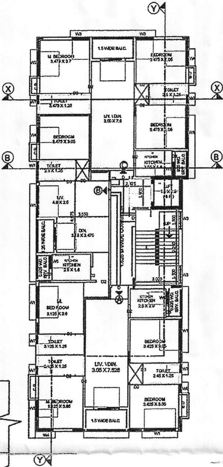
FLOOR 01, FLOOR 02, FLOOR 03, FLOOR 04, FLOOR 05-TYPICAL TYPICAL FLOOR PLAN ( 1ST TO 5TH ) SCALE - 1:1
